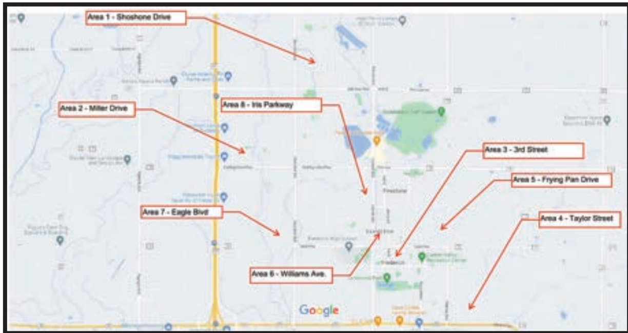
Figure 7.1 Fire Hydrant Test Locations for Hydraulic Model Calibration
